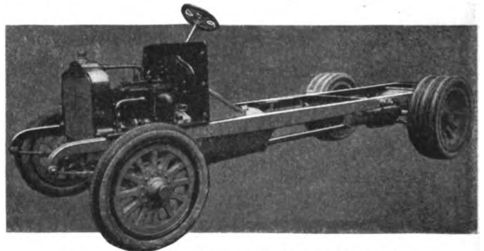
Chassis of Saurer Four-Cylinder Truck En Bloc.
